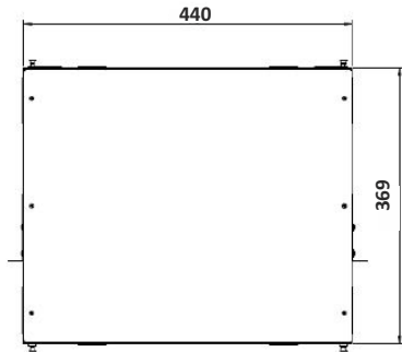
PATCH PANEL
