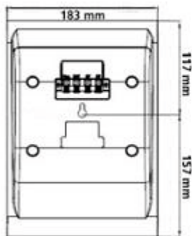
Hanging Hole
