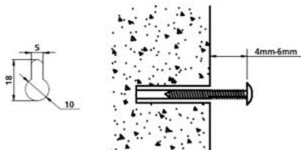
Nail for Mounting
