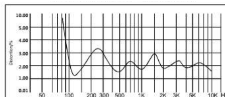
DISTORTION (THD<1.5% 1W, 1m, 100Hz-10kHz)
