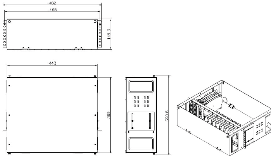
PATCH PANEL
